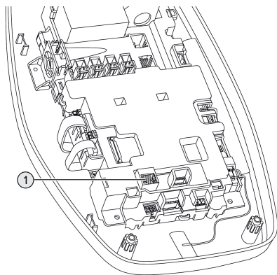
Fig. 14: Porta Ethernet
