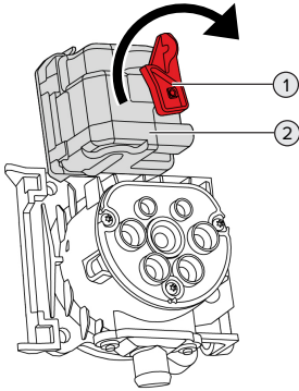
Fig. 25: Unlock the charging plug manually
