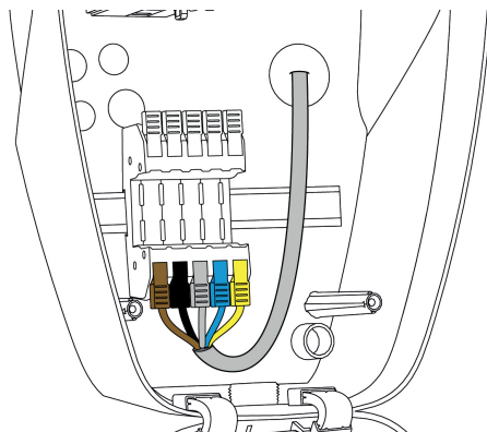
Fig. 10: Power supply connection (example)
