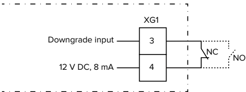
Fig. 17: Schematic circuit diagram: Connection of an external switching contact (default setting: NO)
