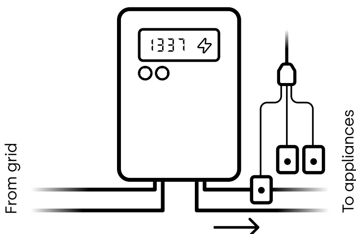
Fig 2. Connection diagram for 1-phase system
