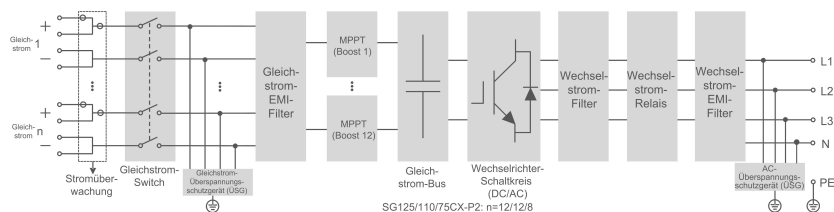
figure 2-4 Schaltplan
