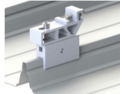
Domico GBS, Rib-Roof 465
