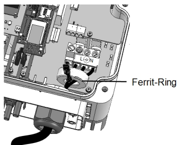
Abbildung 23: AC-Anschlüsse
